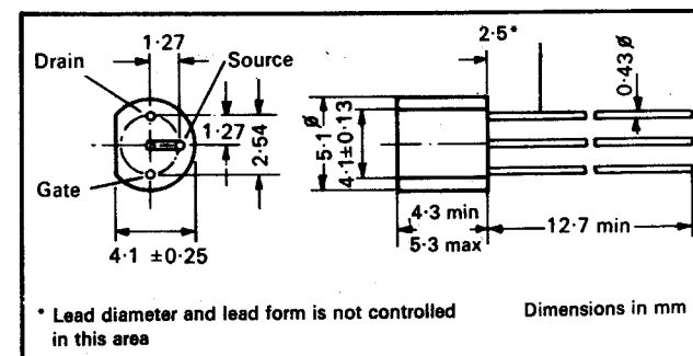
TO-18 pin circle
