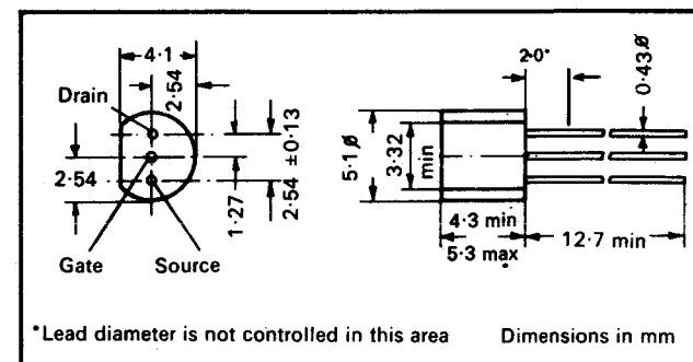
TO-92
